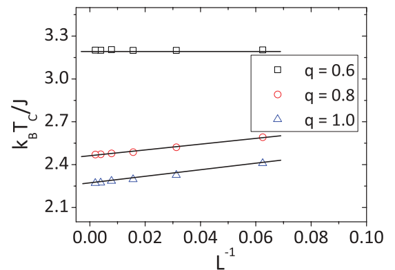
FIG. 2. (Color online) Extrapolation ( L \rightarrow \infty ) of critical temperatures for different q values: 0.6, 0.8, and 1.0 for the 2D Ising model.
