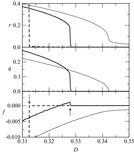
FIG. 2. Order parameters r and q and free energy per site f as functions of D , for c = 8.0 , exhibiting a continuous transition at T = 0.07 (thin solid lines) and a first-order transition at T = 0.04 (thick solid lines for SG states and dashed lines for P states) discussed in the text. The arrows indicate points on the spinodals.
