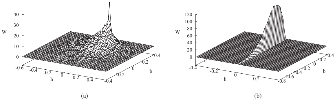
FIG. 1. Local field distribution W(h, b) for c = 6.0 , D = 0.35 , and T = 0.1 , with initial conditions (a) (A) and (b) (B).
