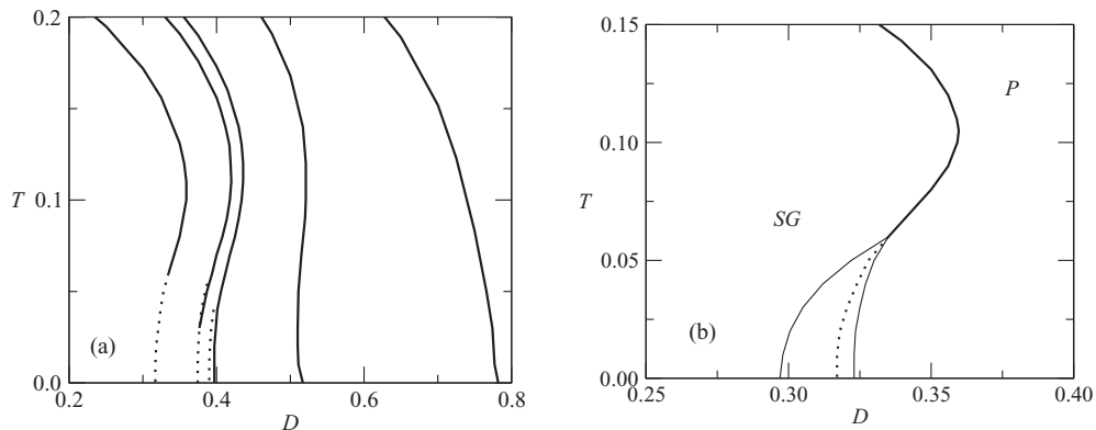
FIG. 3. (a) The T vs D phase diagram for connectivity c = 2.0, 4.0, 5.6, 6.0 , and 8.0 , from right to left. Solid (dotted) lines denote continuous (discontinuous) transitions between a spin-glass (SG) phase to the left and a paramagnetic (P) phase to the right of each curve. (b) Detail of the phase boundary for c = 8 , including the spinodals of the P and SG phases to the left and right of the transition as thin solid lines, respectively.
