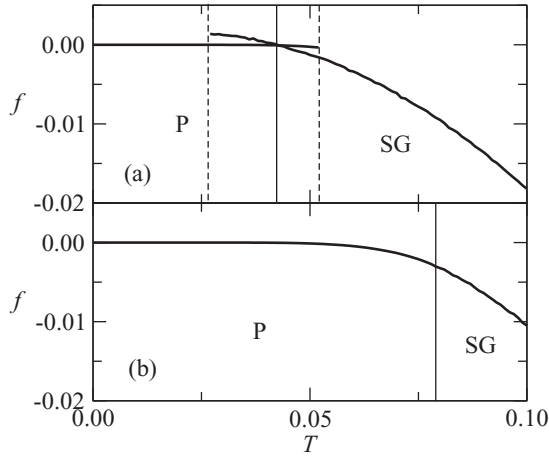
FIG. 4. Temperature dependence of the free energy for c = 8 across (a) the first-order transition at D = 0.325 and (b) the continuous transition at D = 0.35 . The dashed left (right) line indicates a point on the SG (P) spinodals, and the vertical solid lines indicate the transition with an increase in entropy from the P phase to the SG phase in (a) and with no increase in (b). The normal transition between the SG and P phases (not shown) appears at higher T .
