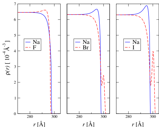
FIG. 3 (color online). Density profiles for NaF, NaBr, and NaI at 1M concentration. The GDS is at r = 300 \text{ \AA} .
