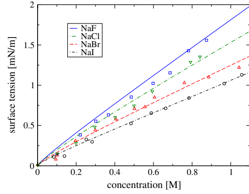
FIG. 2 (color online). Surface tension of NaF, NaCl, NaBr, and NaI. \text{Na}^{+} and \text{Cl}^{-} are partially hydrated with a_h = 2.5 Å and 2.0 Å, respectively, \text{F}^{-} is fully hydrated with a_h = 3.52 Å, while the large halogens \text{I}^{-} and \text{Br}^{-} are unhydrated. Symbols are the experimental data from [25].
