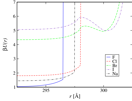
FIG. 1 (color online). The ion-surface interaction potentials at 1M salt concentration. For hydrated ions there is a hardcore repulsion from the GDS located at r = 300 Å, and the cavitation energy is omitted since it is constant.
