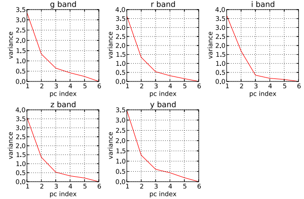
Figure 8. Value of the variance of the principal components as a function of their index for the five (per-band) PCAs performed on the six types of magnitudes: mag_auto , mag_iso , mag_model , mag_petro , mag_spheroid and mag_psf .
