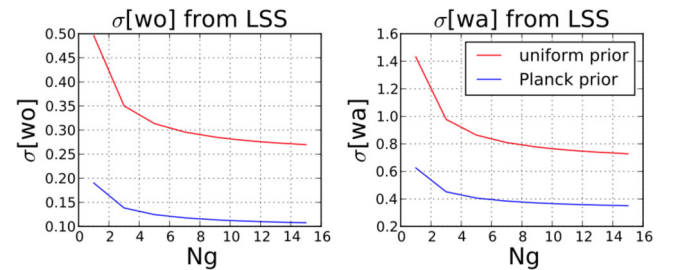
Figure 2. Marginalized statistical errors on the equation-of-state parameters w_o and w_a from the LSS probe, for different values of the density of detected galaxies N_g . The errors are marginalized over \{\Omega_m, H, \sigma_8, \Omega_b, n_s, b_g\} and computed using the same assumptions and setup as in the WL case (see Section 3.2.1), with l \in [10, 400] , to avoid the non-linear regime and following most recent l -cuts work by the LSS community (Rassat et al. 2008; Audren et al. 2013). The red curve shows the errors computed with a non-informative prior whereas the blue curve is obtained assuming a Planck prior.
