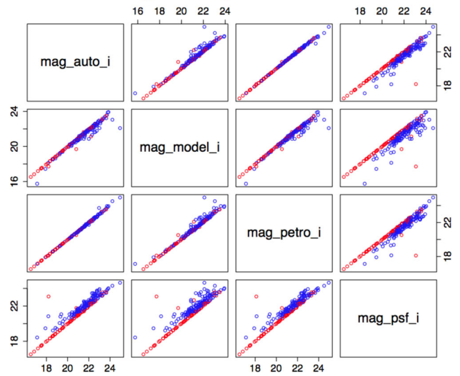
Figure 7. Scatter plots for stars (red markers) and galaxies (blue markers) for four different types of magnitudes in the i band. The magnitudes are strongly correlated and PCA is therefore well adapted to re-express them in a new basis of independent variables.
